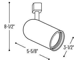
NTH-105B Black Roundback Cylinder with Black Baffle
