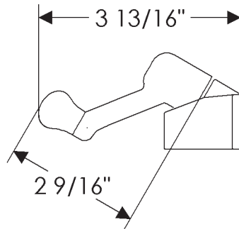
WC160 Casement Window Hardware Crank & Cover
