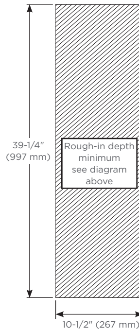
Rough-in Dimensions
